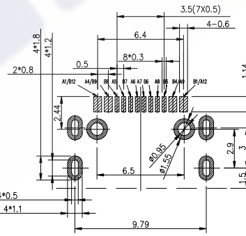
RECOMMENDED P.C.B. LAYOUT TOLERANCE UNSPECIFIED ±0.05mm
