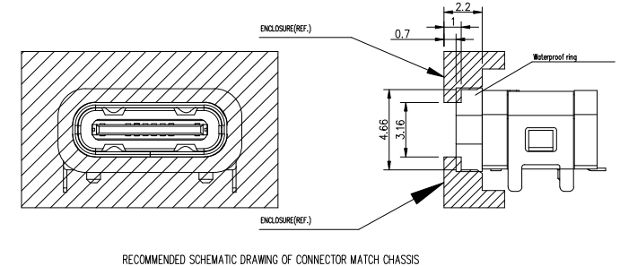
RECOMMENDED SCHEMATIC DRAWING OF CONNECTOR MATCH CHASSIS
