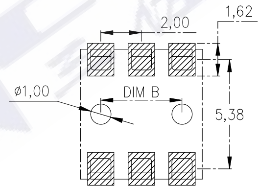
RECOMMENDED PCB LAYOUT TOP VIEW(.XX±0.05)
