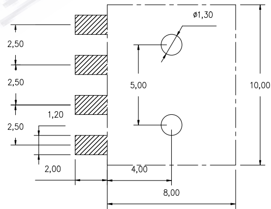
RECOMMENDED PCB LAYOUT TOP VIEW(.XX±0.05)
